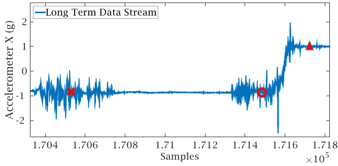
Fig. 10. Stand-to-Sit start times for outlier. The x marks the start based on the MoST template and the circle marks the start based on the data specific template. The triangle marks the end of the movement for both templates.
