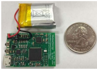
Fig. 2. Custom sensor board with 3-axis accelerometer, 3-axis gyroscope, and TI MSP430 used for data collection.
