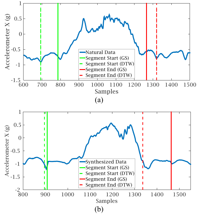
Fig. 9. Segmentation of movements for natural data (a) and synthesized data (b) from subject 3 for the grasp from shelf movement on the arm sensor. The gold standard is based on visual annotation (natural) or tool annotation (synthesized).
