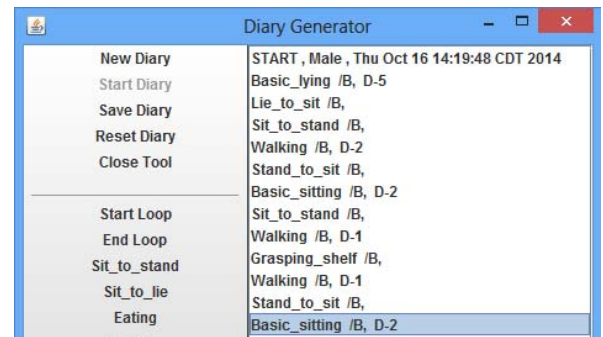
Fig. 5. Diary Generator tool which allows the user to input a sequence of movements and options based on the database.
