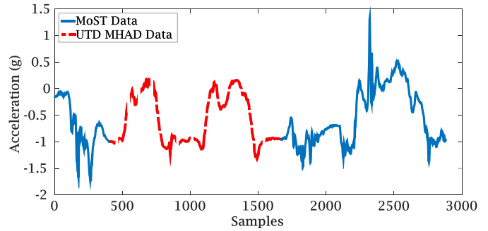
Fig. 11. Synthesis of wrist sensor data from MoST and UTD MHAD.
