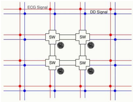
Figure 9: Network Topology
