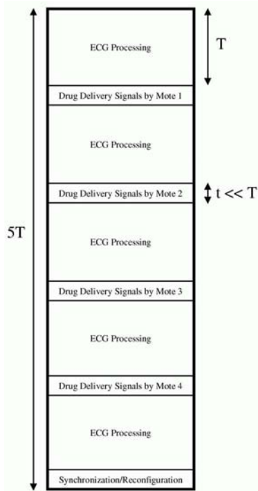
Figure 10: Task Multiplexing in Medical Jacket Network
