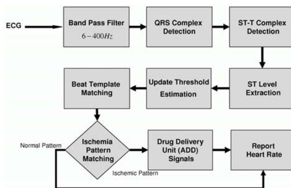
Figure 8: Ischemia Detection Operations
