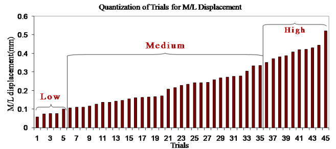
Figure 7. M/L displacement measured from acceleration data and quantized into three classes
