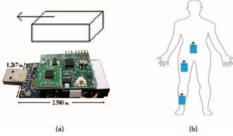
Figure 3: (a) TelsoB mote (b) Placement of the notes
